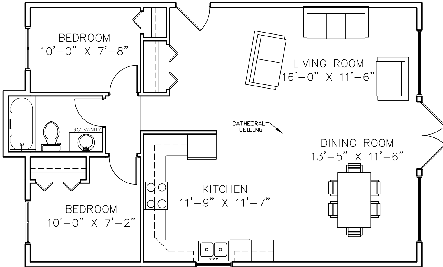
MAIN FLOOR - 876 SQ FT
