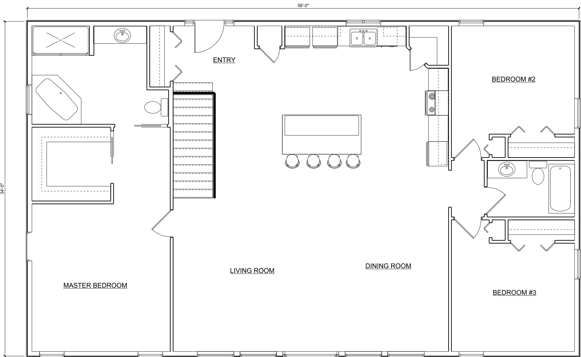
MAIN FLOOR 1925 sq/ft
